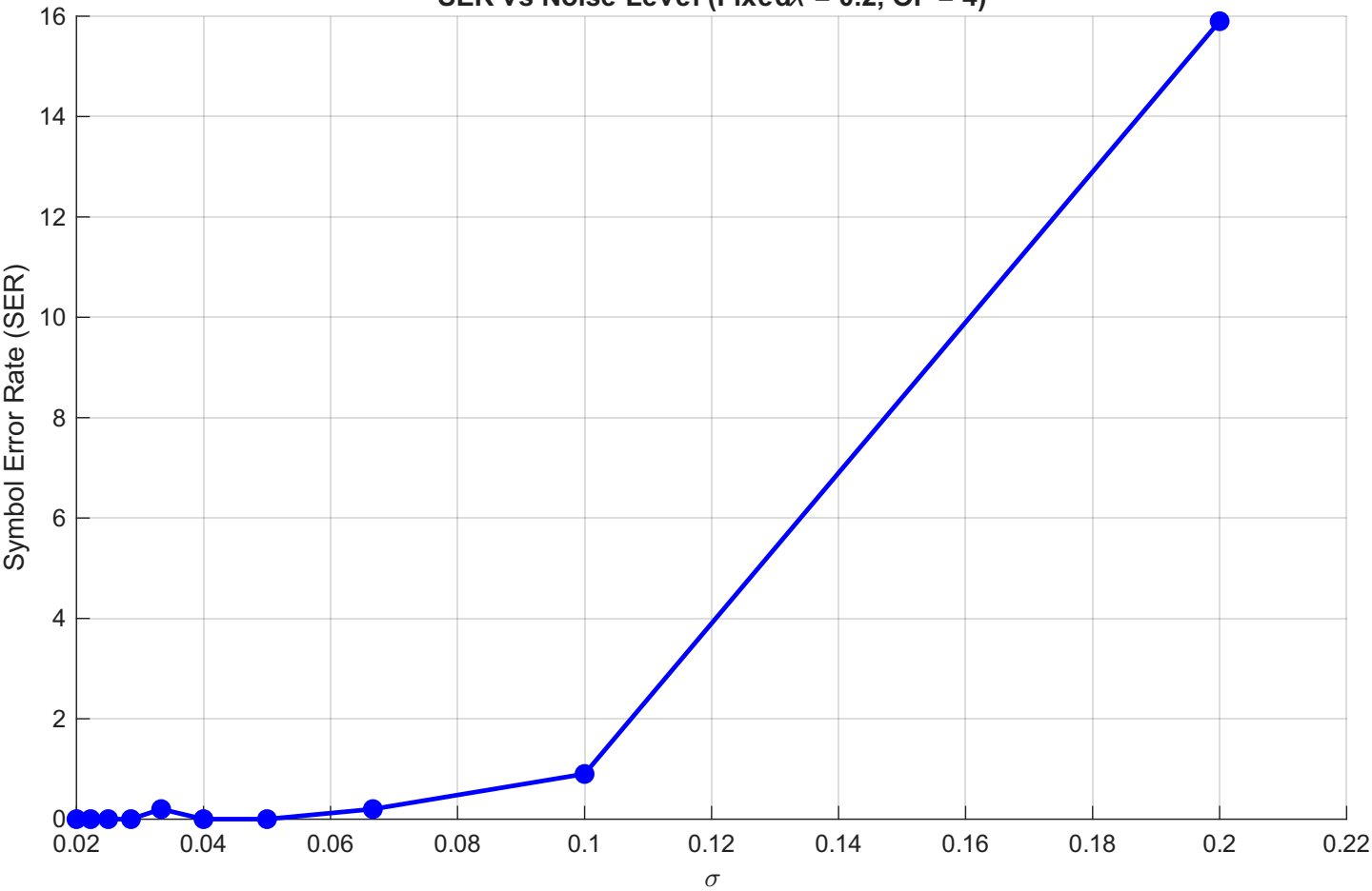
SER vs Noise Level (Fixed \lambda = 0.2 , OF = 4)
